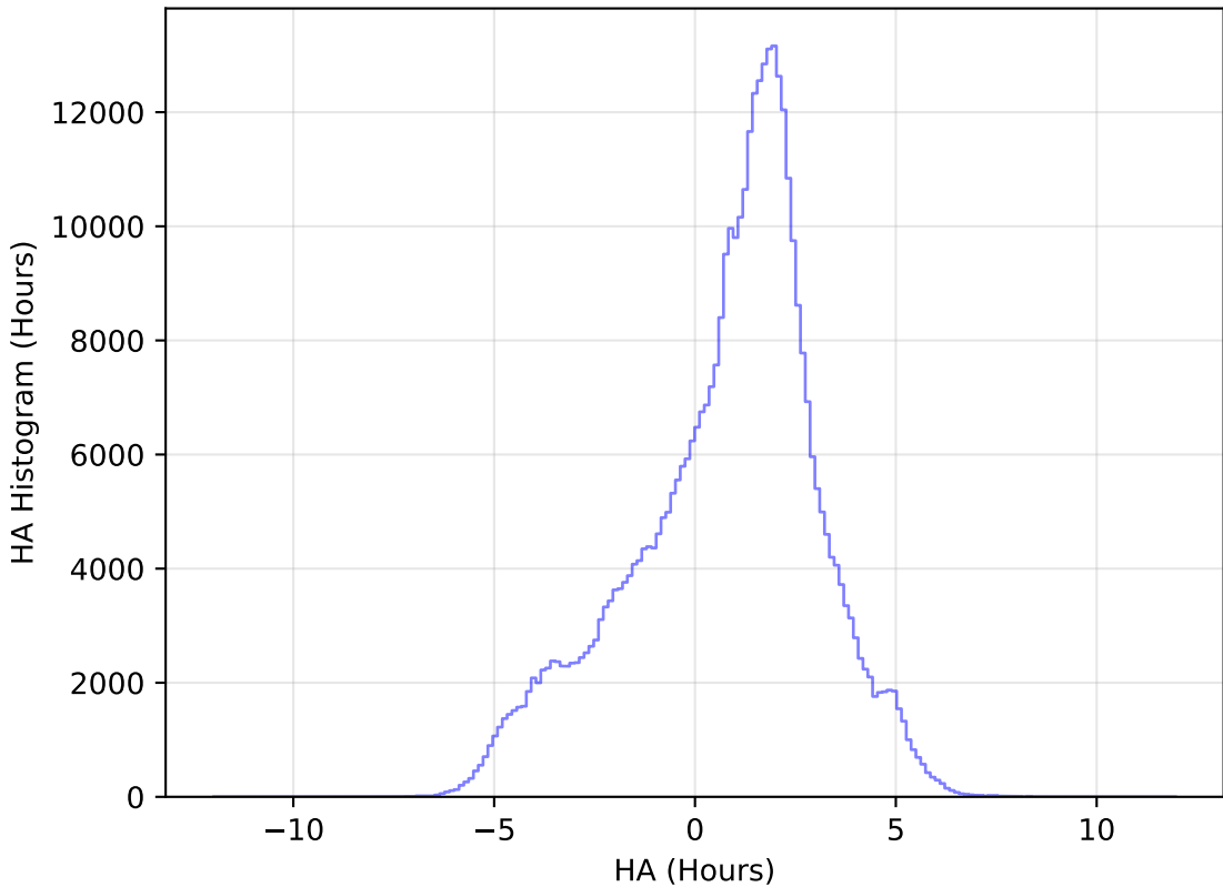
too_elab_heavy_r32_d2_griz_v3.4_10yrs WFD z band: HA Histogram
