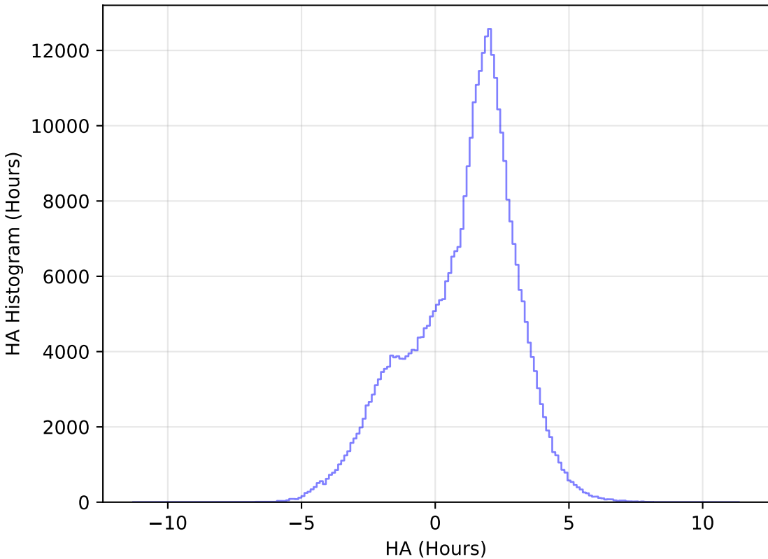
too_elab_heavy_r32_d2_griz_v3.4_10yrs WFD y band: HA Histogram
