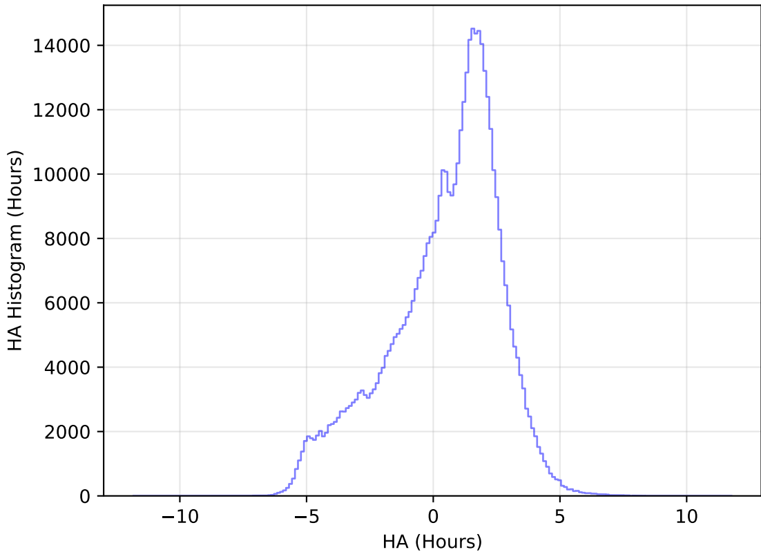
too_elab_heavy_r32_d2_griz_v3.4_10yrs WFD r band: HA Histogram
