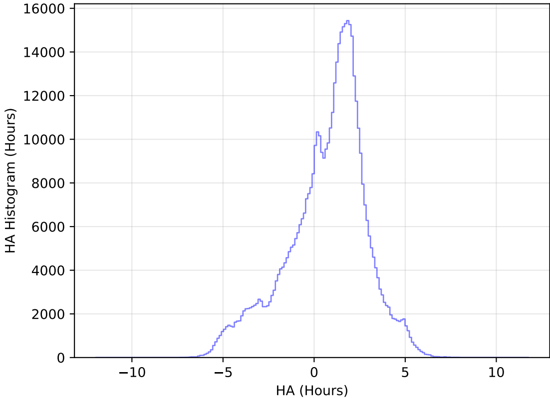
too_elab_heavy_r32_d2_griz_v3.4_10yrs WFD i band: HA Histogram
