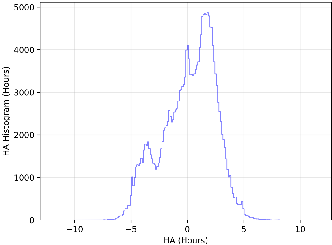
too_elab_heavy_r32_d2_griz_v3.4_10yrs WFD g band: HA Histogram
