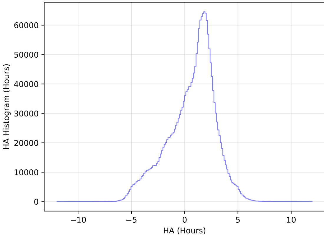
too_elab_heavy_r32_d2_griz_v3.4_10yrs WFD all bands: HA Histogram
