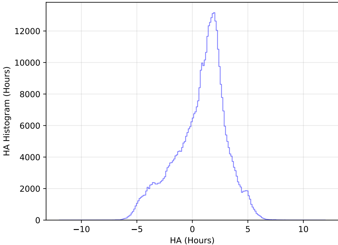
too_elab_heavy_r32_d2_griz_v3.4_10yrs All sky z band: HA Histogram
