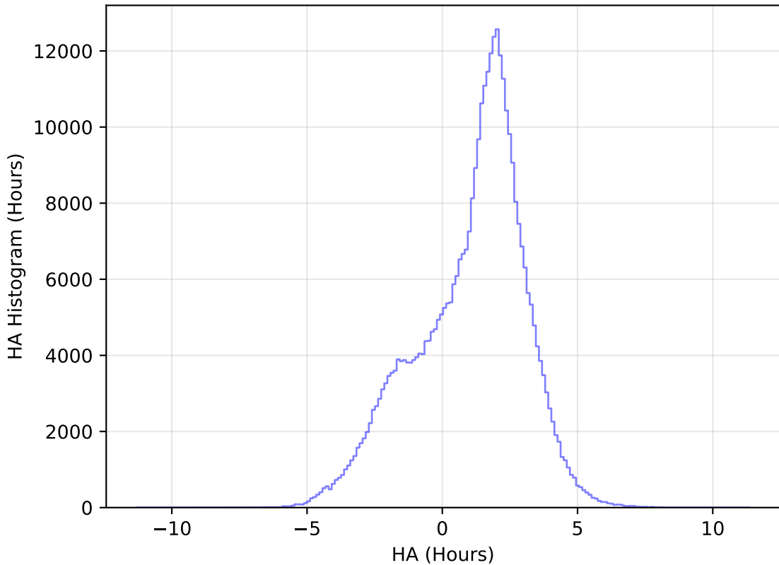
too_elab_heavy_r32_d2_griz_v3.4_10yrs All sky y band: HA Histogram
