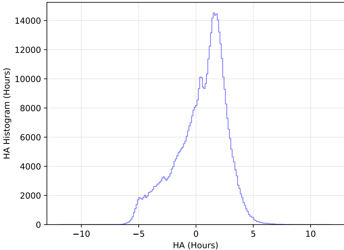
too_elab_heavy_r32_d2_griz_v3.4_10yrs All sky r band: HA Histogram
