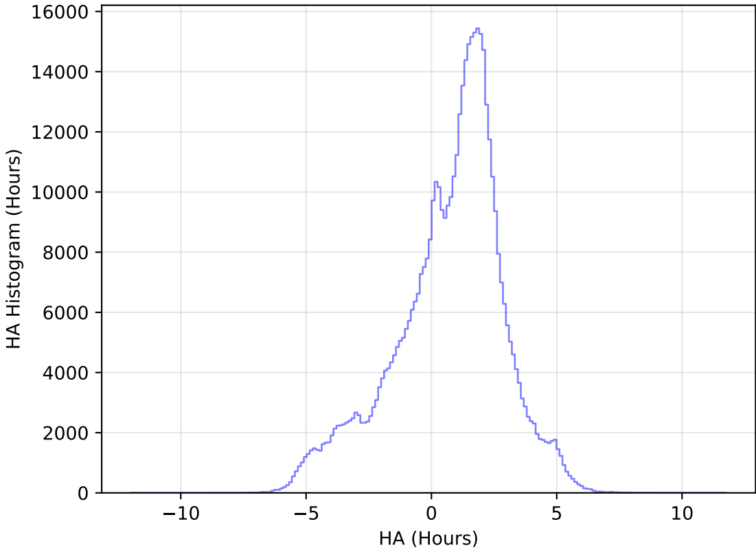
too_elab_heavy_r32_d2_griz_v3.4_10yrs All sky i band: HA Histogram
