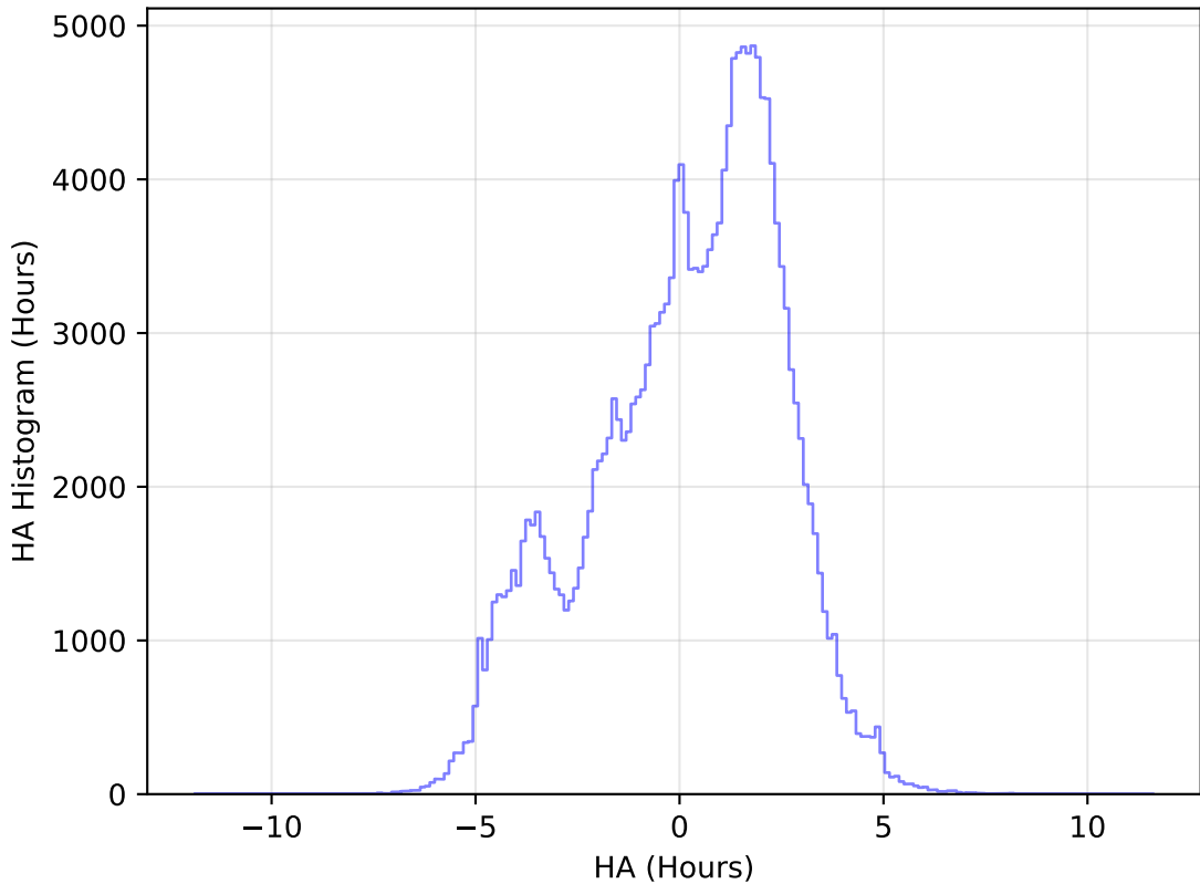
too_elab_heavy_r32_d2_griz_v3.4_10yrs All sky g band: HA Histogram
