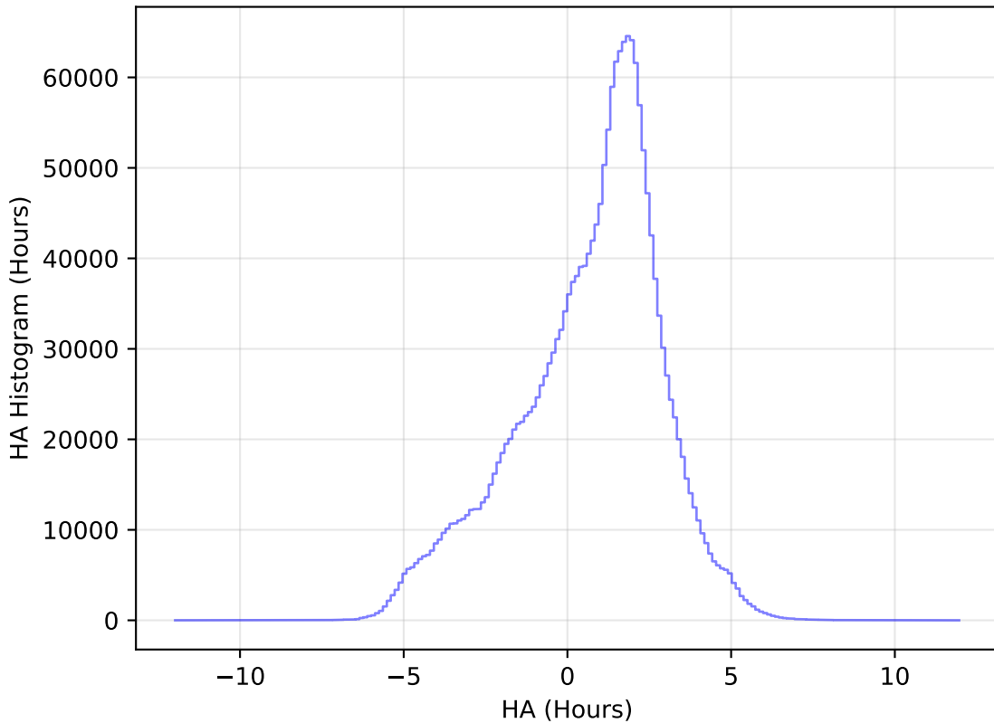
too_elab_heavy_r32_d2_griz_v3.4_10yrs All sky all bands: HA Histogram
