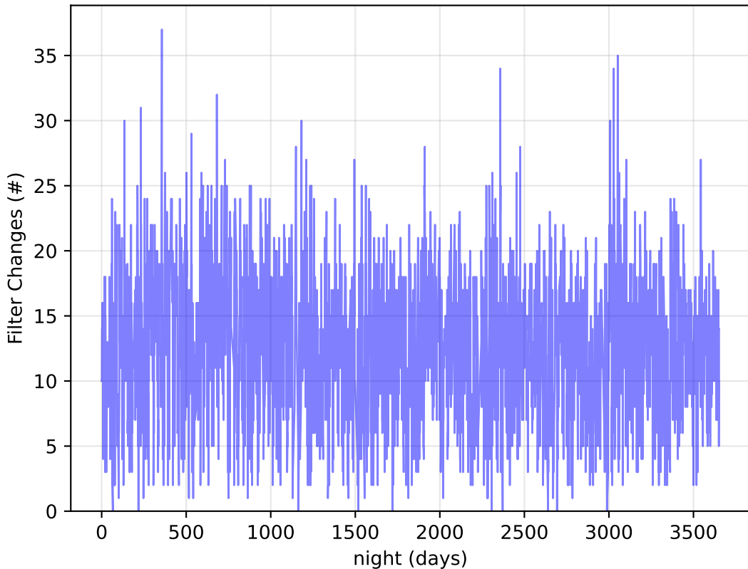
too_elab_heavy_r32_d2_griz_v3.4_10yrs Per Night: Filter Changes
