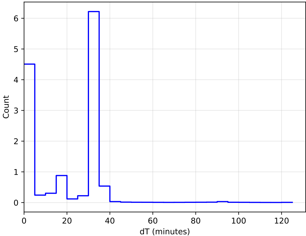
too_elab_heavy_r32_d2_griz_v3.4_10yrs All sky: DeltaT Histogram 1e6
