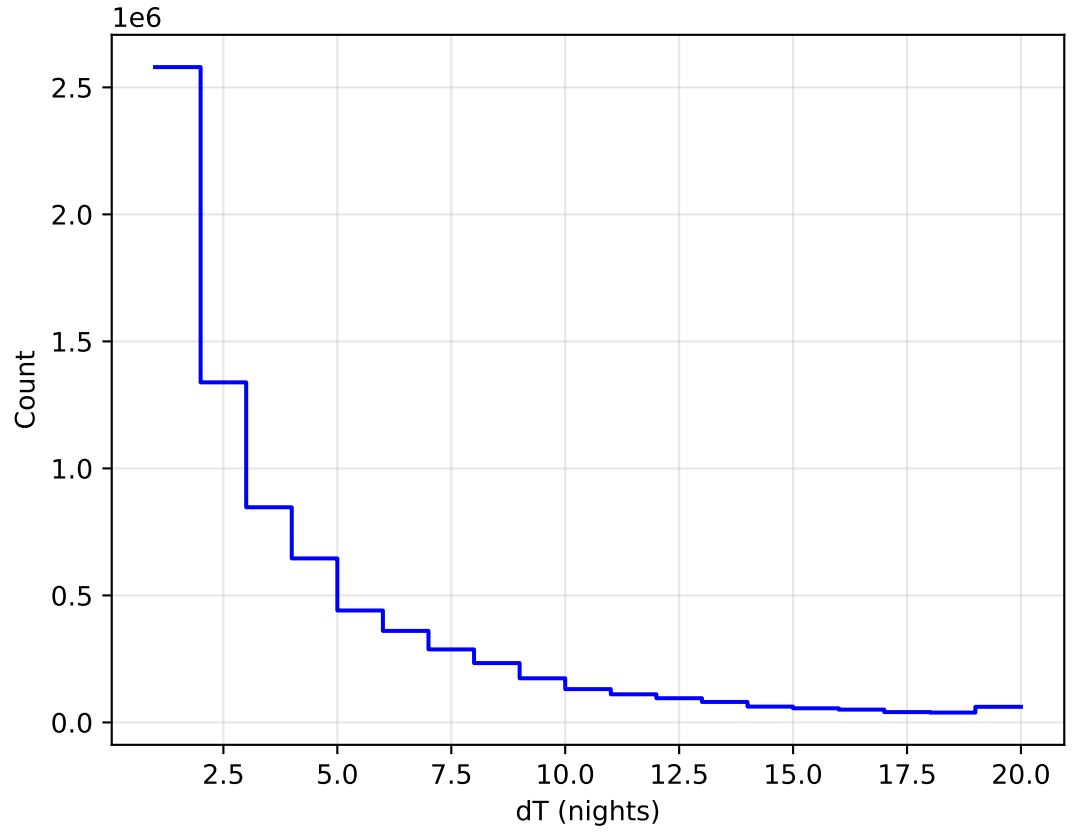
too_elab_heavy_r32_d2_griz_v3.4_10yrs WFD all bands: DeltaNight Histogram
