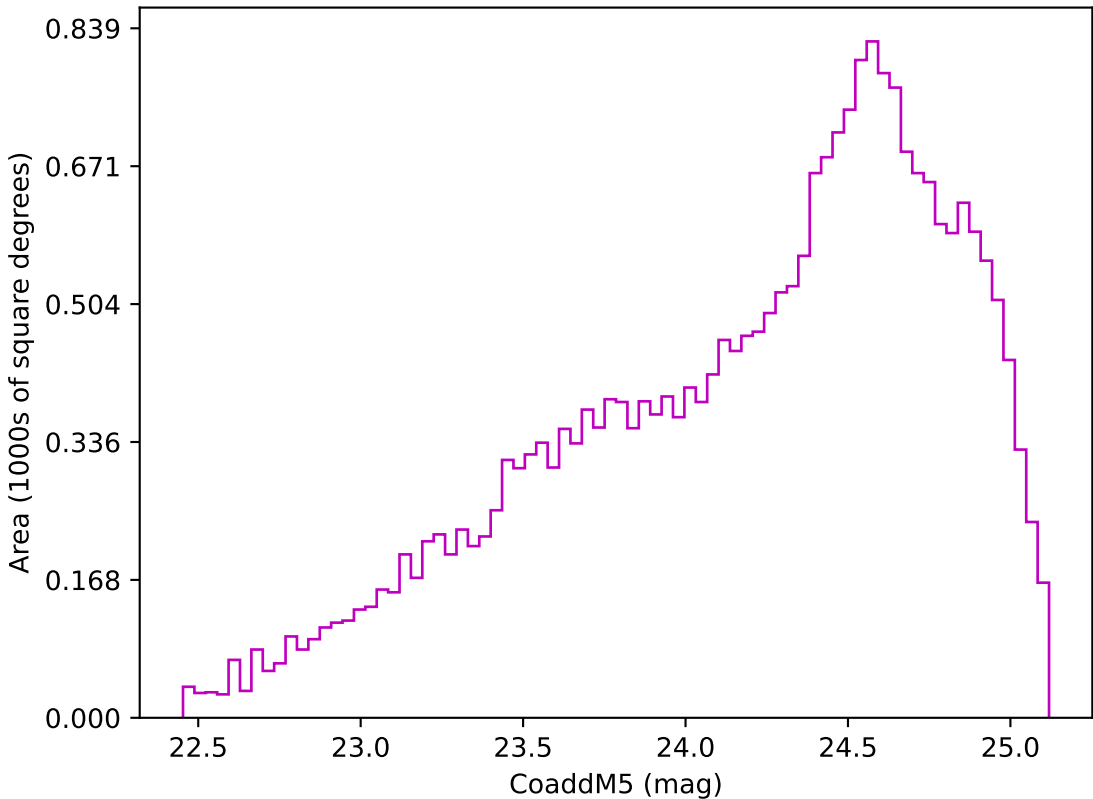
too_elab_heavy_r32_d2_griz_v3.4_10yrs Yr 3-4 z band: CoaddM5
