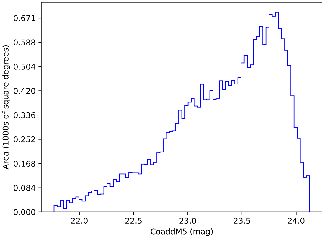
too_elab_heavy_r32_d2_griz_v3.4_10yrs Yr 3-4 y band: CoaddM5
