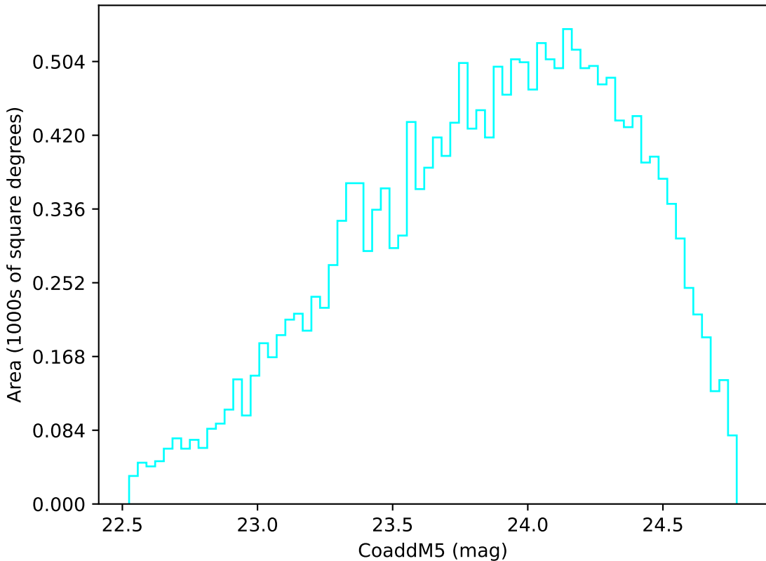
too_elab_heavy_r32_d2_griz_v3.4_10yrs Yr 3-4 u band: CoaddM5
