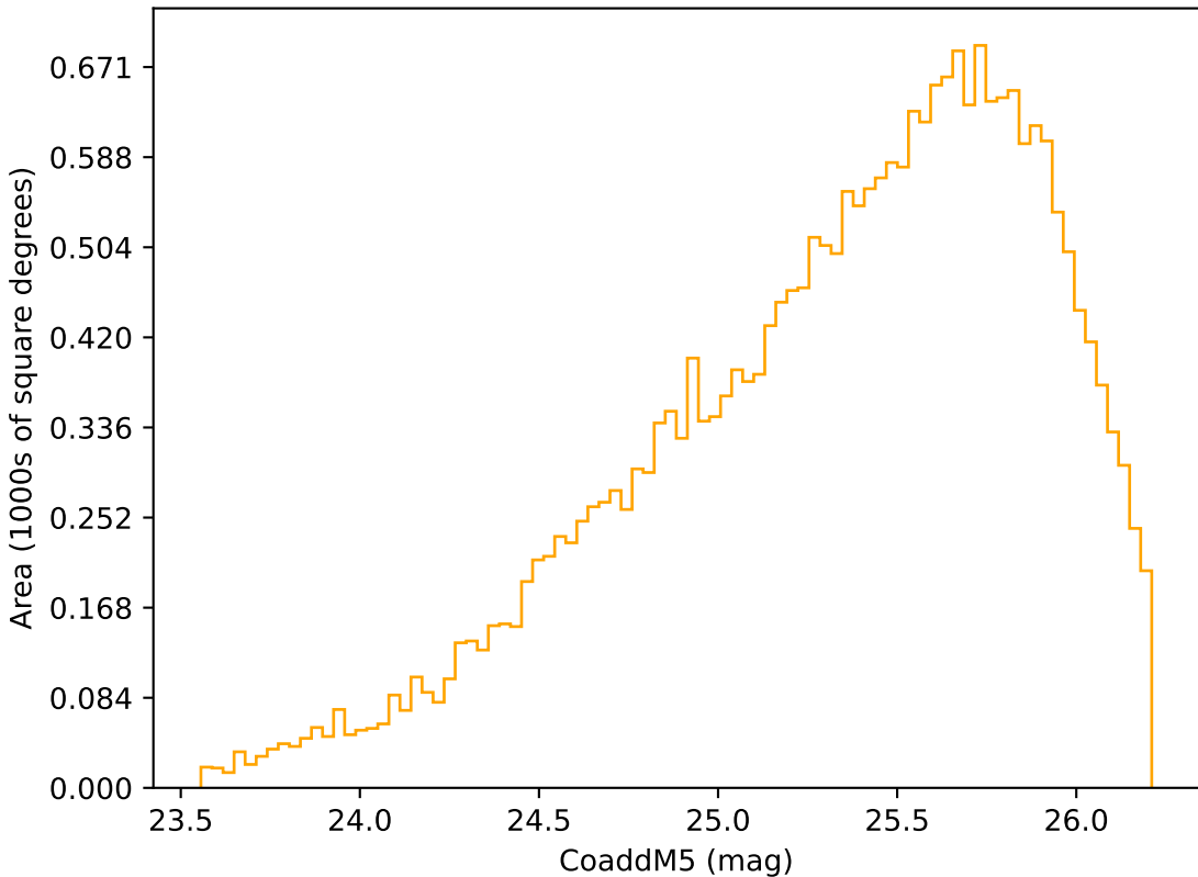
too_elab_heavy_r32_d2_griz_v3.4_10yrs Yr 3-4 r band: CoaddM5
