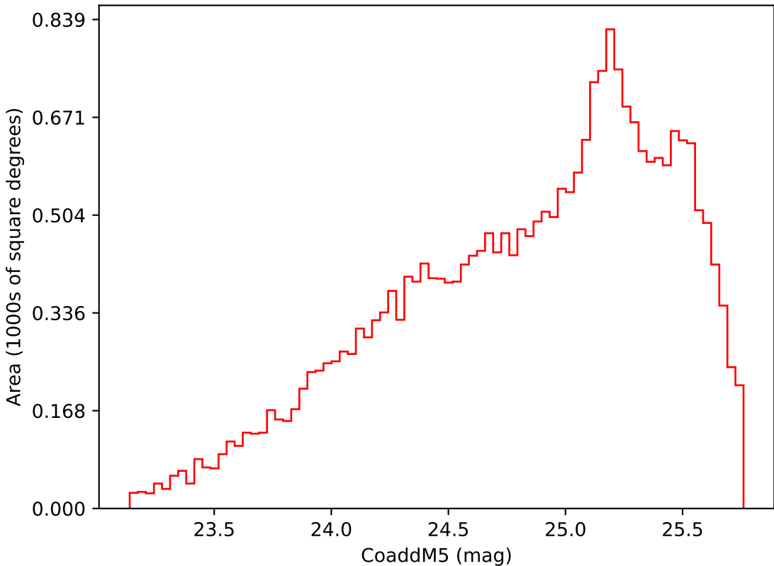
too_elab_heavy_r32_d2_griz_v3.4_10yrs Yr 3-4 i band: CoaddM5
