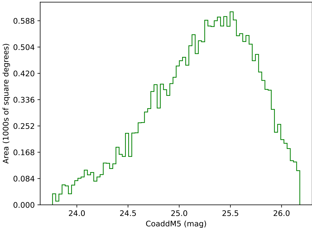
too_elab_heavy_r32_d2_griz_v3.4_10yrs Yr 3-4 g band: CoaddM5
