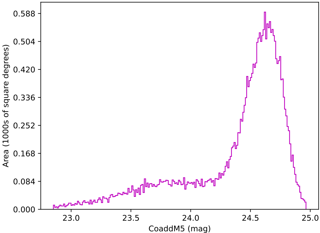
too_elab_heavy_r32_d2_griz_v3.4_10yrs Yr 1 z band: CoaddM5
