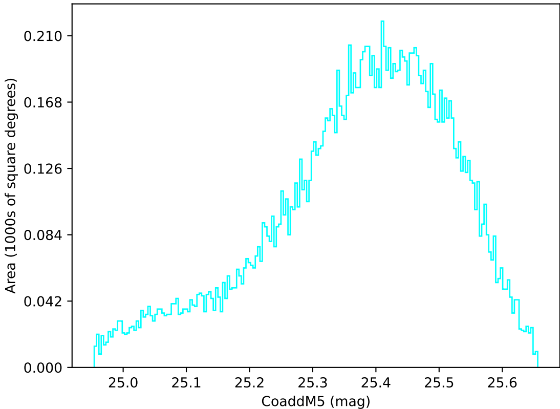
too_elab_heavy_r32_d2_griz_v3.4_10yrs WFD u band: CoaddM5
