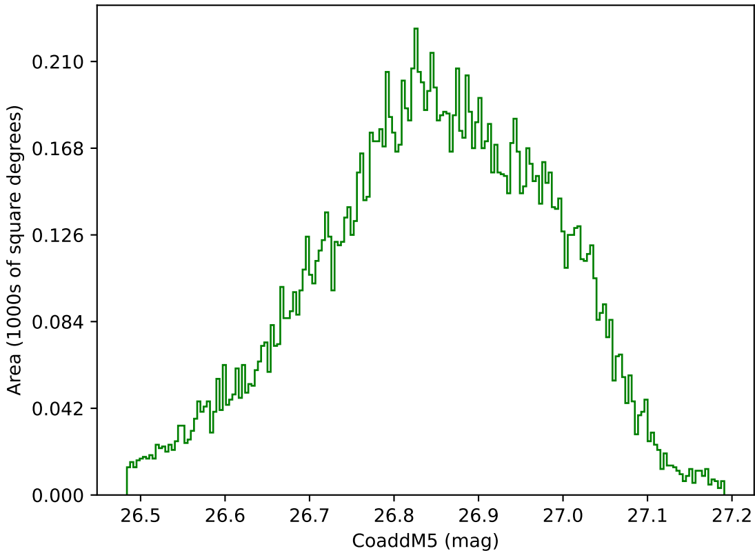
too_elab_heavy_r32_d2_griz_v3.4_10yrs WFD g band: CoaddM5
