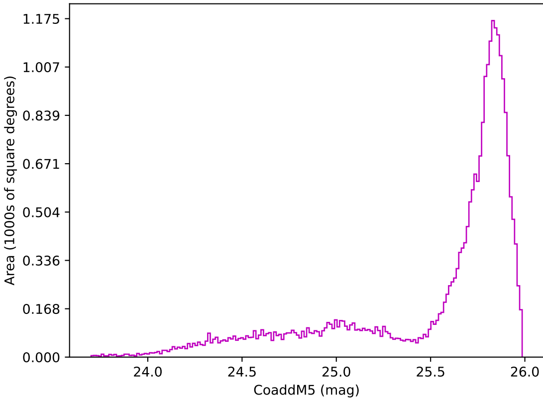
too_elab_heavy_r32_d2_griz_v3.4_10yrs All sky z band: CoaddM5
