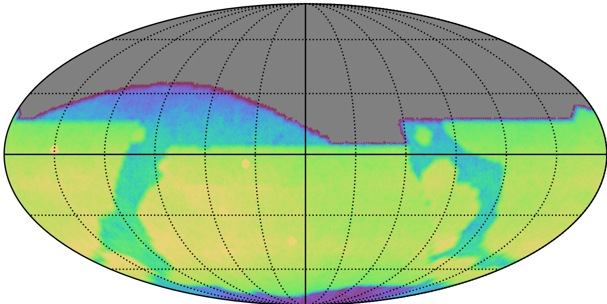
too_elab_heavy_r32_d2_griz_v3.4_10yrs All sky r band: CoaddM5
