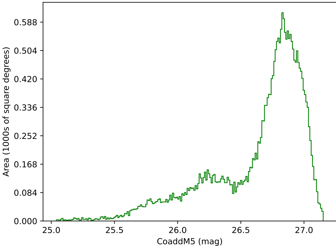
too_elab_heavy_r32_d2_griz_v3.4_10yrs All sky g band: CoaddM5
