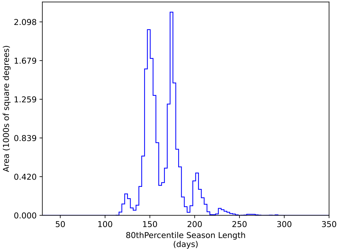
too_elab_heavy_r32_d2_griz_v3.4_10yrs WFD y band: 80thPercentile Season Length
