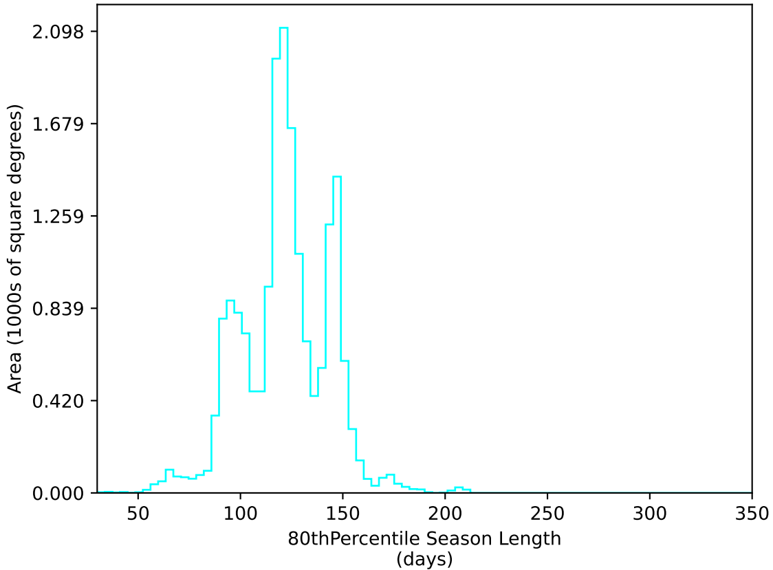
too_elab_heavy_r32_d2_griz_v3.4_10yrs WFD u band: 80thPercentile Season Length
