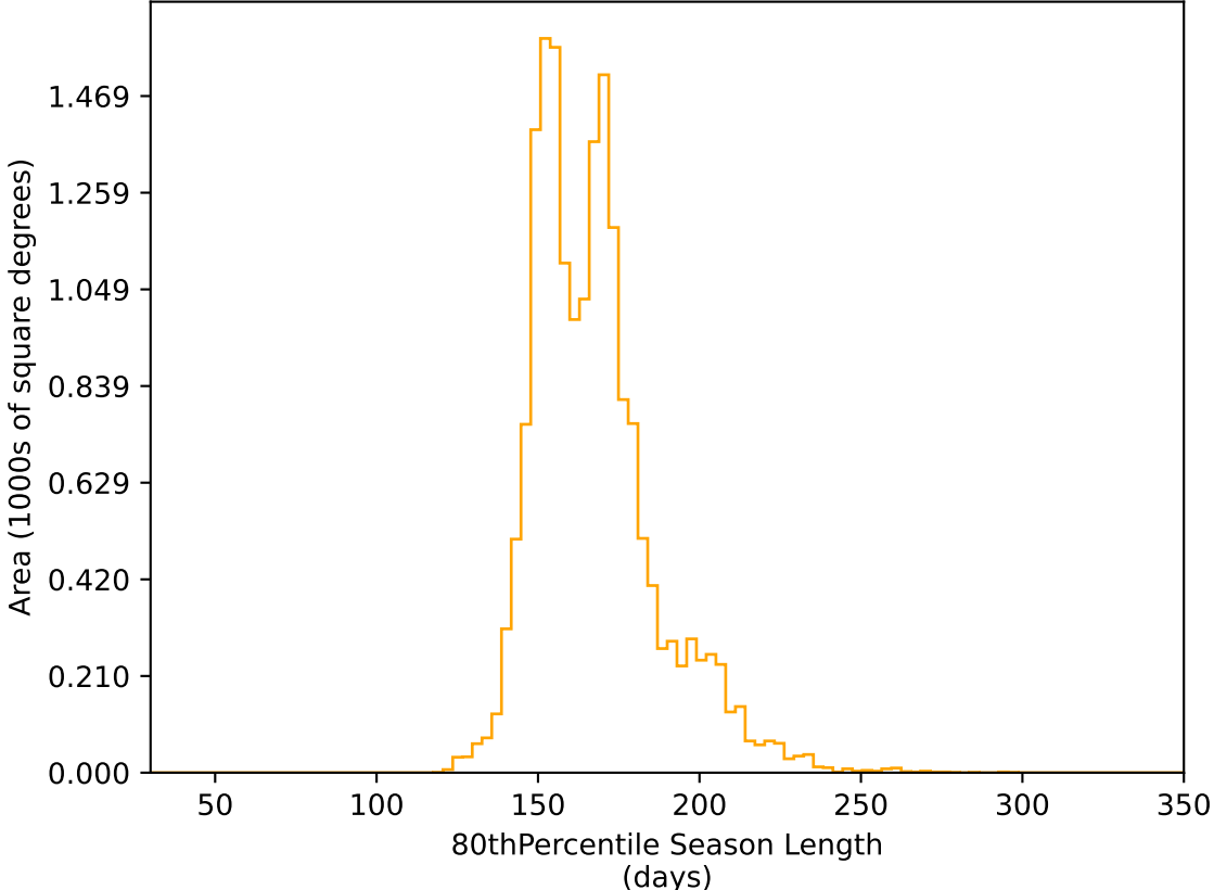
too_elab_heavy_r32_d2_griz_v3.4_10yrs WFD r band: 80thPercentile Season Length
