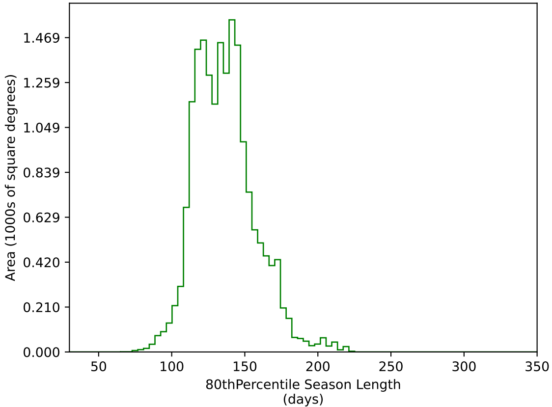
too_elab_heavy_r32_d2_griz_v3.4_10yrs WFD g band: 80thPercentile Season Length
