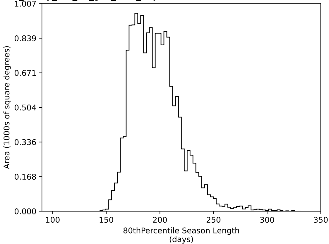
too_elab_heavy_r32_d2_griz_v3.4_10yrs WFD all bands: 80thPercentile Season Length
