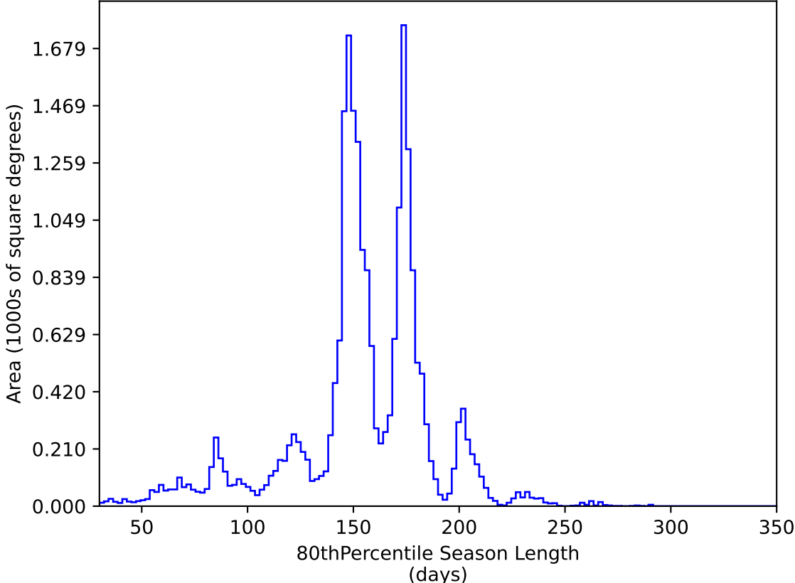
too_elab_heavy_r32_d2_griz_v3.4_10yrs All sky y band: 80thPercentile Season Length
