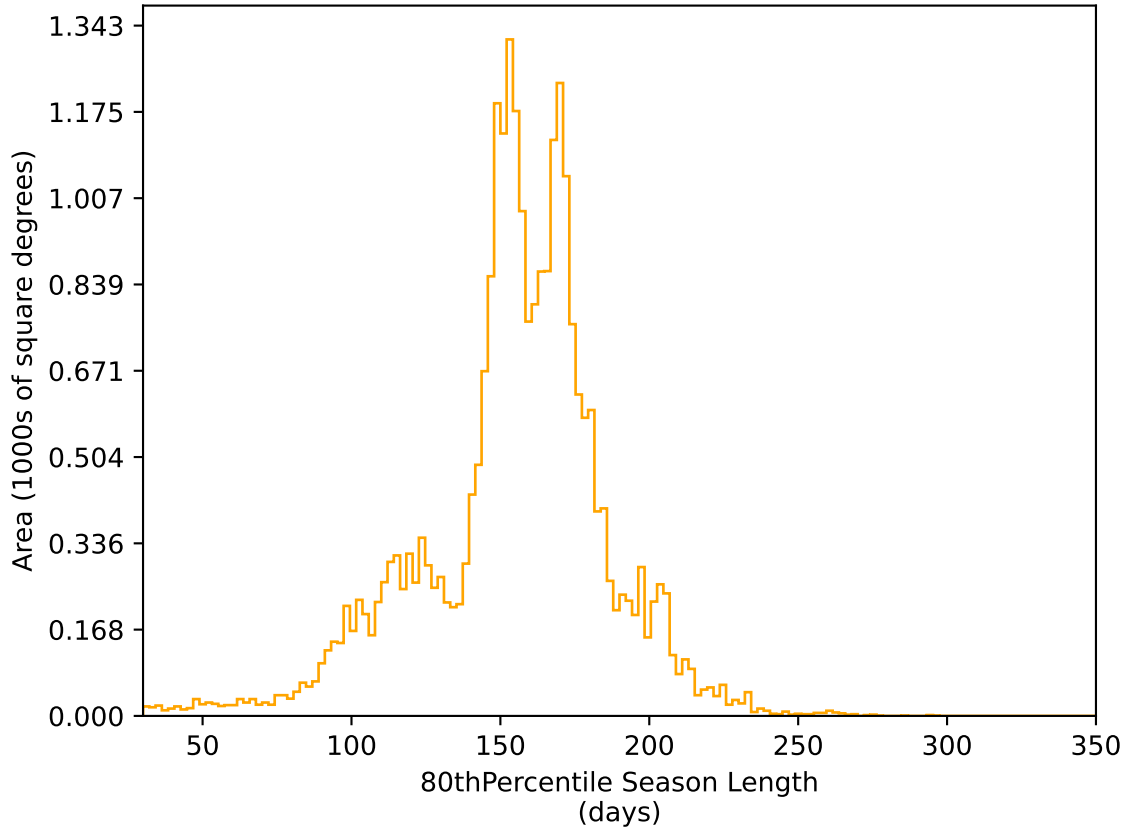
too_elab_heavy_r32_d2_griz_v3.4_10yrs All sky r band: 80thPercentile Season Length
