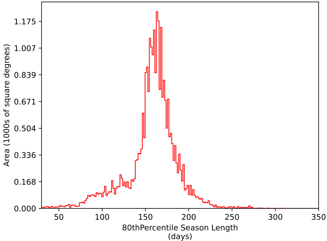
too_elab_heavy_r32_d2_griz_v3.4_10yrs All sky i band: 80thPercentile Season Length
