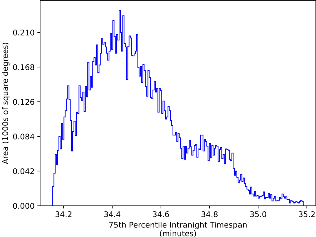
too_elab_heavy_r32_d2_griz_v3.4_10yrs WFD zy bands: 75th Percentile Intranight Timespan
