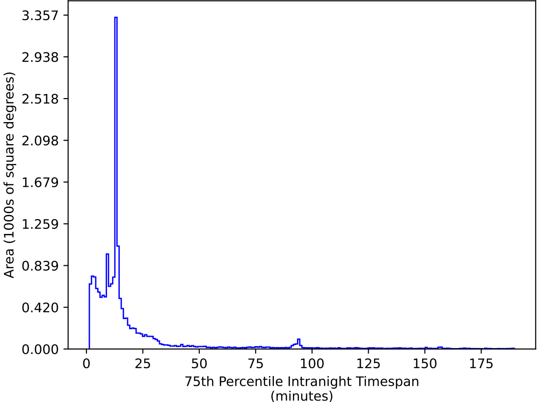
too_elab_heavy_r32_d2_griz_v3.4_10yrs WFD z band: 75th Percentile Intranight Timespan
