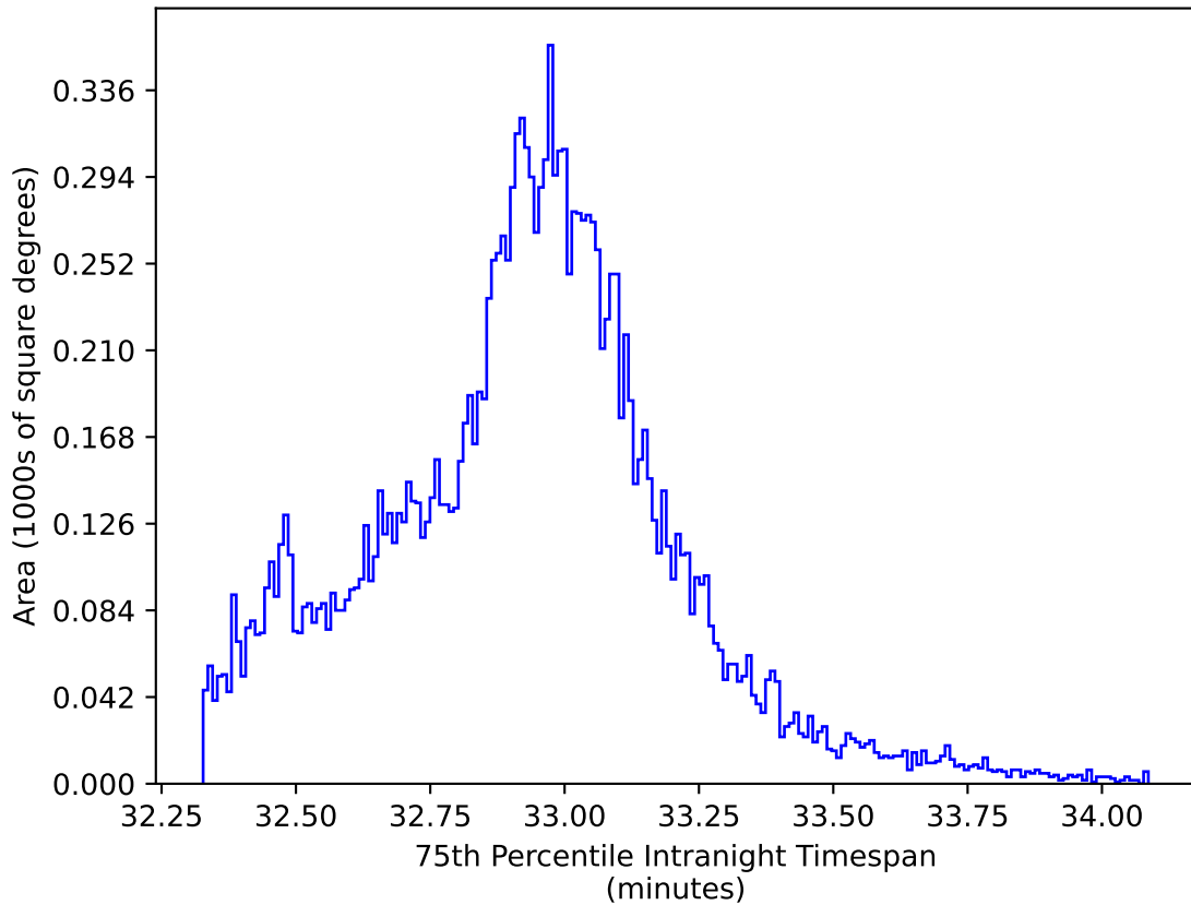
too_elab_heavy_r32_d2_griz_v3.4_10yrs WFD y band: 75th Percentile Intranight Timespan
