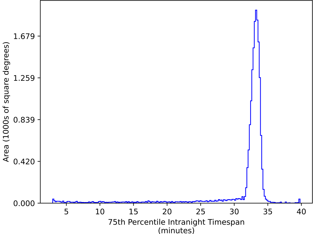
too_elab_heavy_r32_d2_griz_v3.4_10yrs WFD ug bands: 75th Percentile Intranight Timespan
