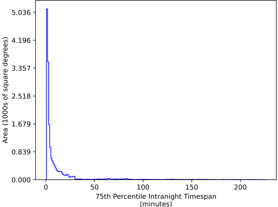
too_elab_heavy_r32_d2_griz_v3.4_10yrs WFD u band: 75th Percentile Intranight Timespan
