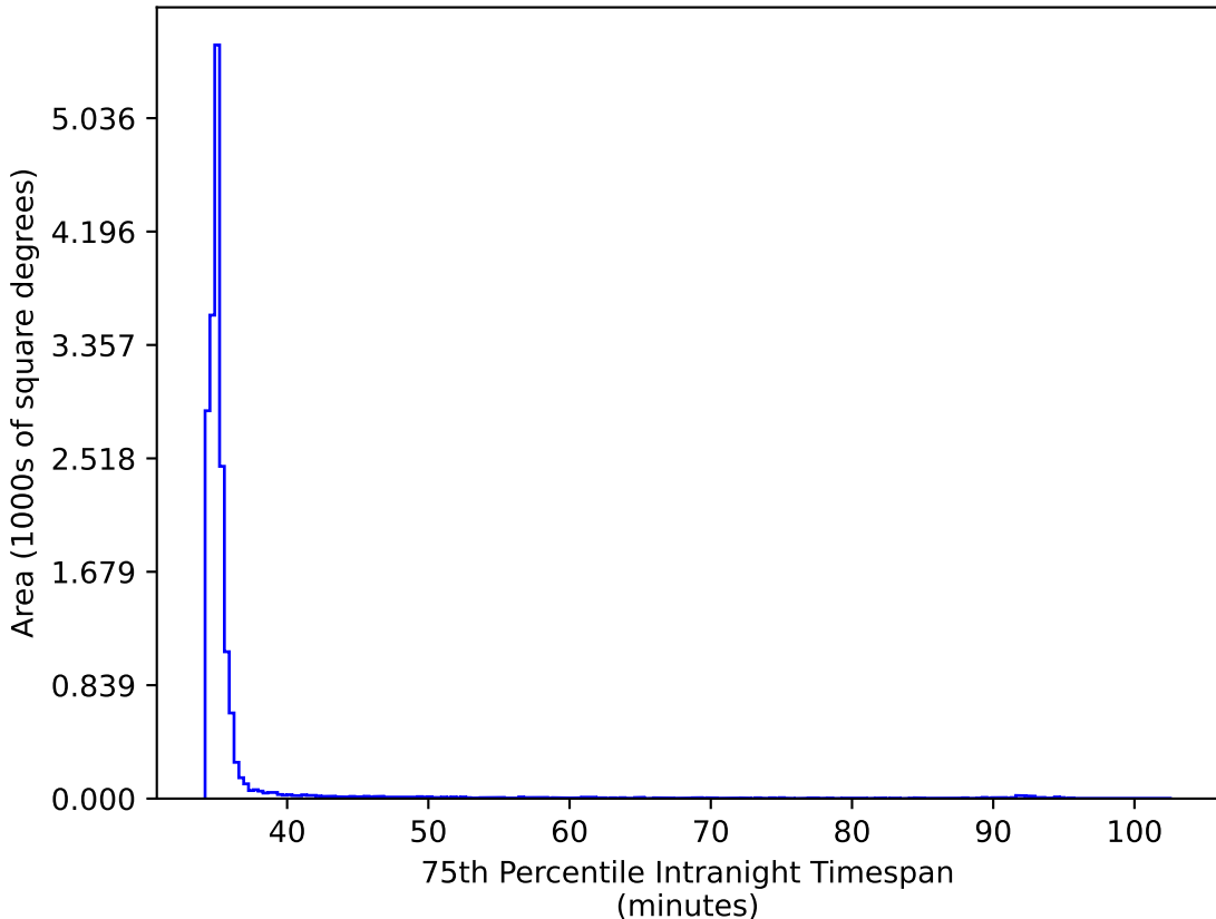
too_elab_heavy_r32_d2_griz_v3.4_10yrs WFD ri bands: 75th Percentile Intranight Timespan
