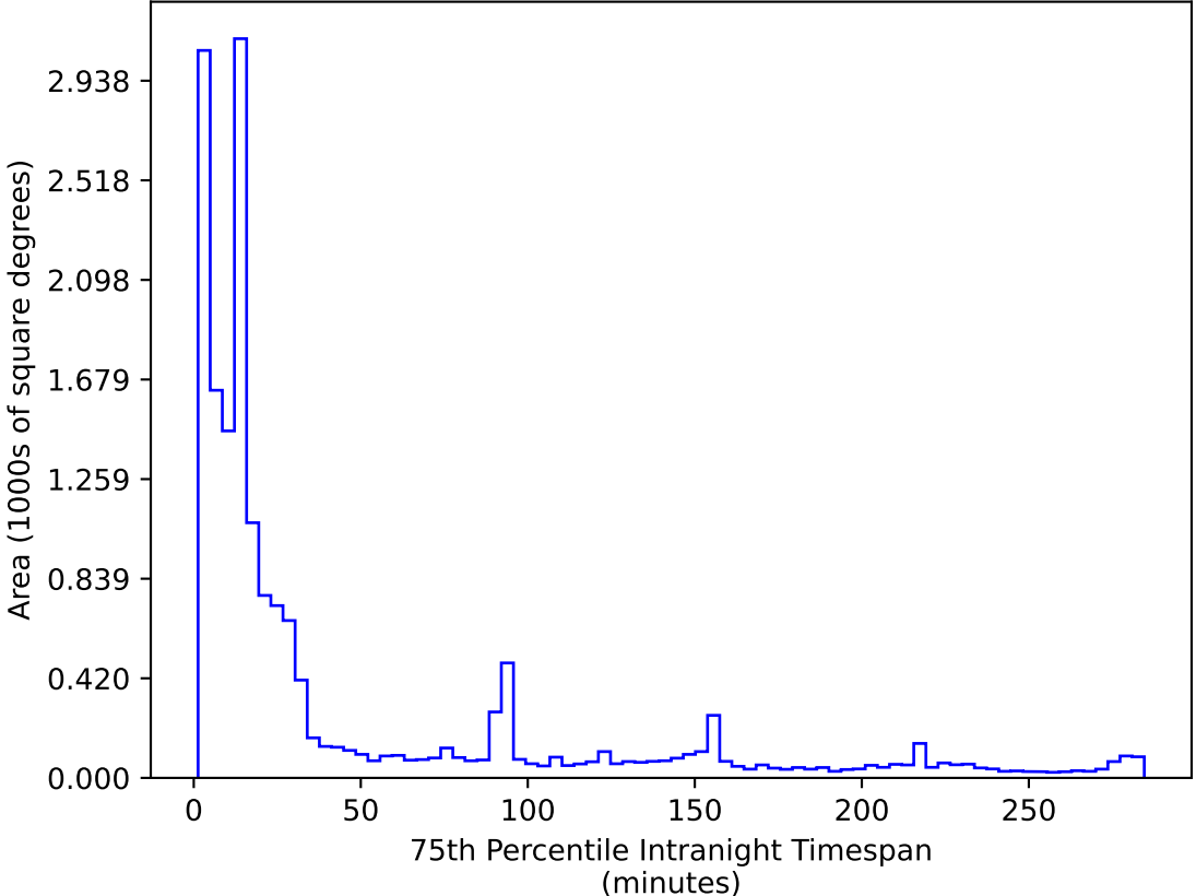
too_elab_heavy_r32_d2_griz_v3.4_10yrs WFD r band: 75th Percentile Intranight Timespan
