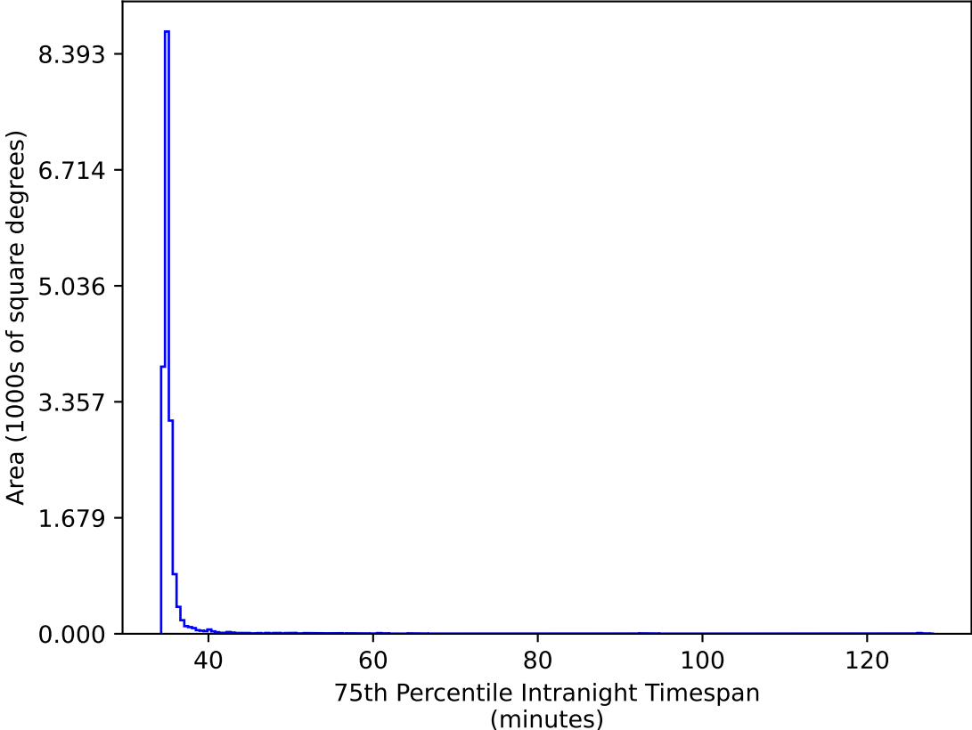
too_elab_heavy_r32_d2_griz_v3.4_10yrs WFD gr bands: 75th Percentile Intranight Timespan
