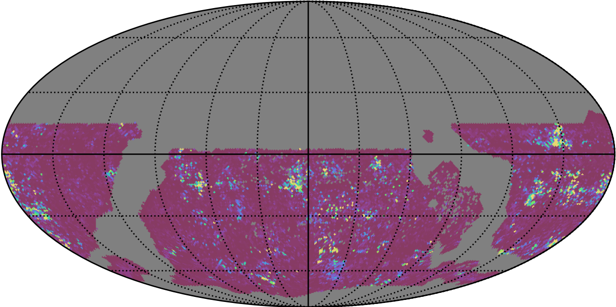
too_elab_heavy_r32_d2_griz_v3.4_10yrs WFD g band: 75th Percentile Intranight Timespan
