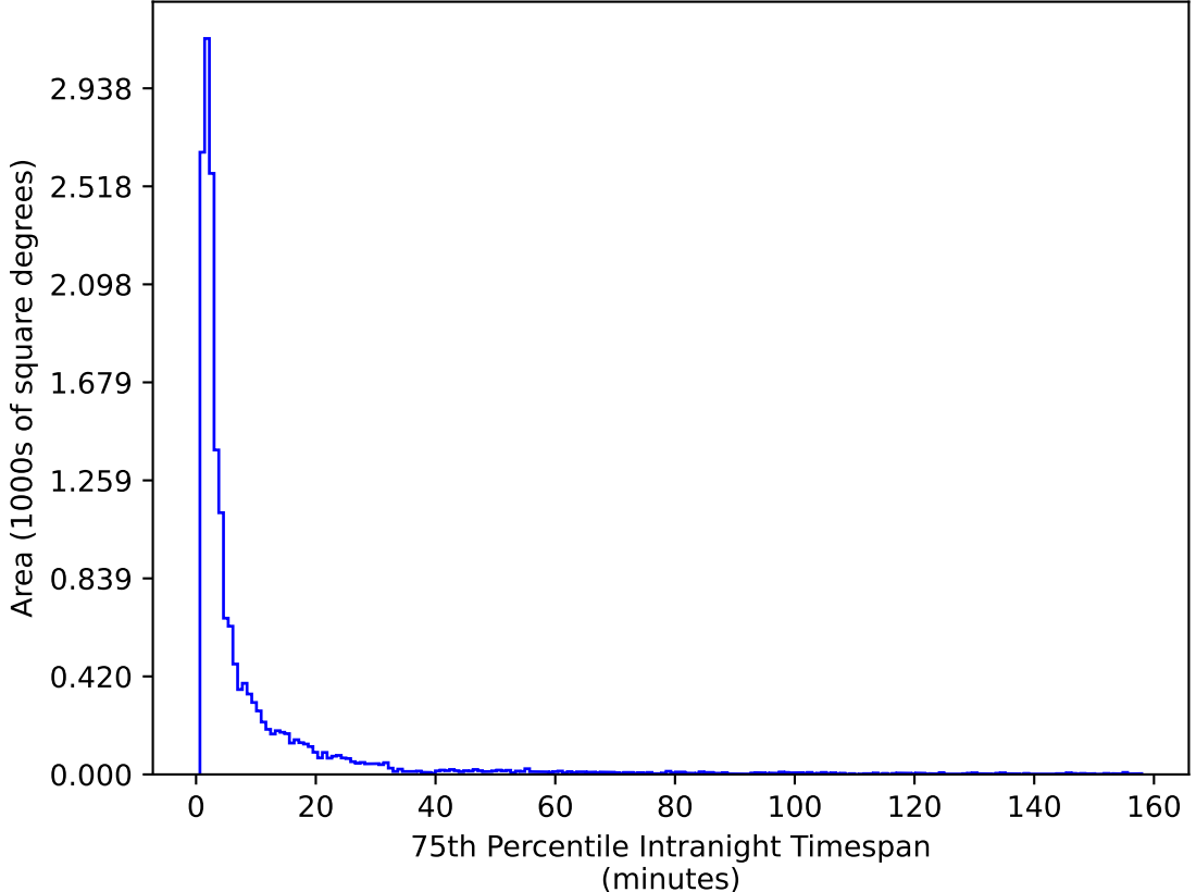
too_elab_heavy_r32_d2_griz_v3.4_10yrs WFD g band: 75th Percentile Intranight Timespan
