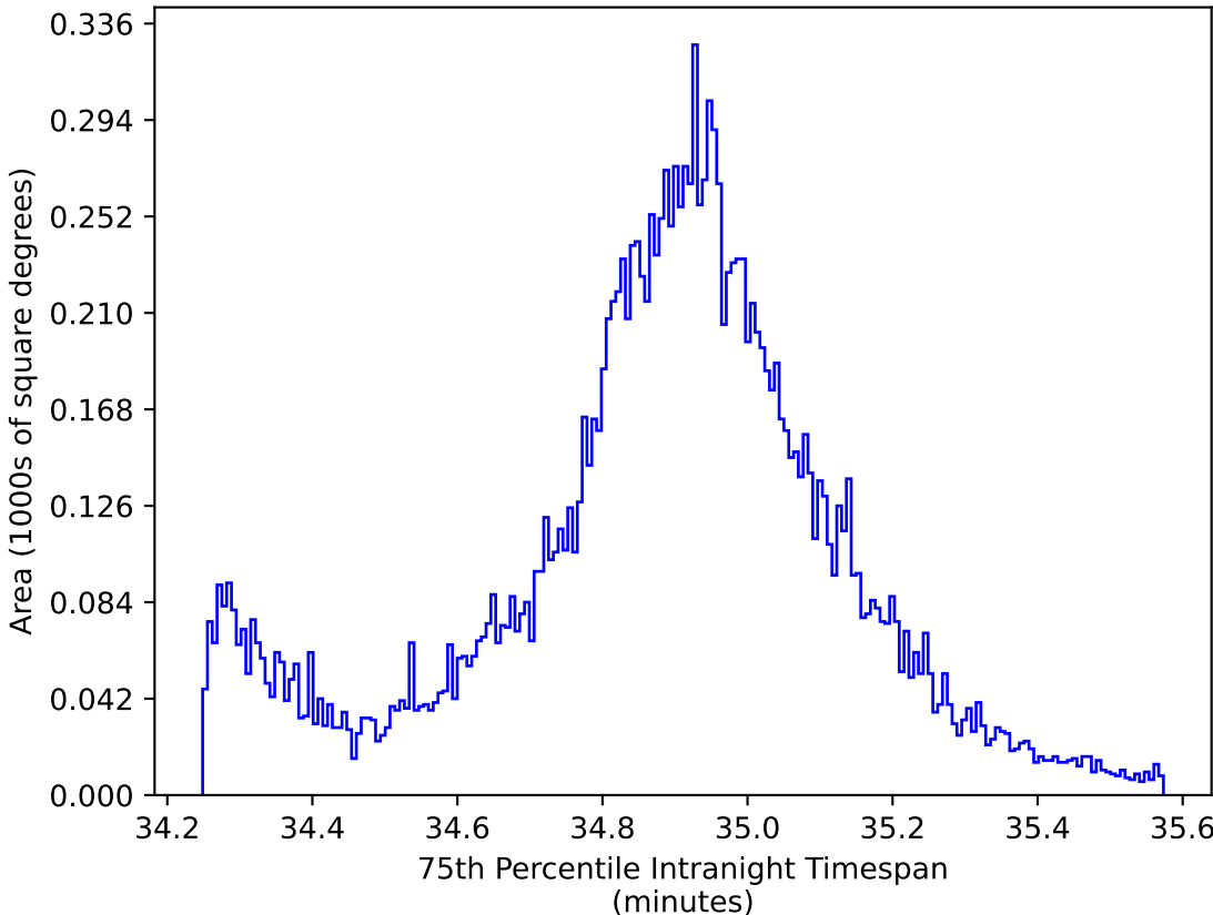
too_elab_heavy_r32_d2_griz_v3.4_10yrs WFD all bands: 75th Percentile Intranight Timespan
