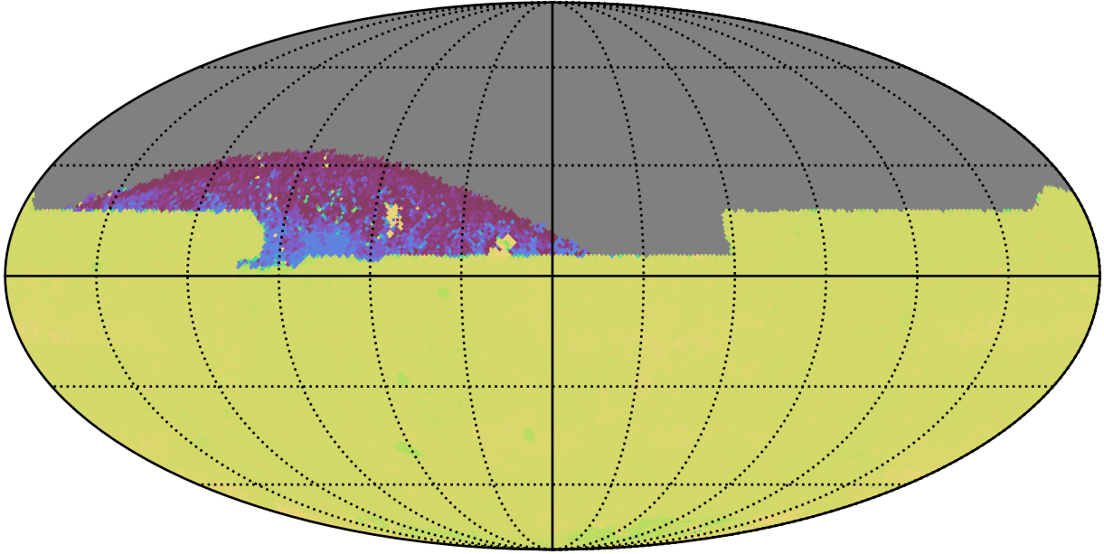
too_elab_heavy_r32_d2_griz_v3.4_10yrs All sky zy bands: 75th Percentile Intranight Timespan
