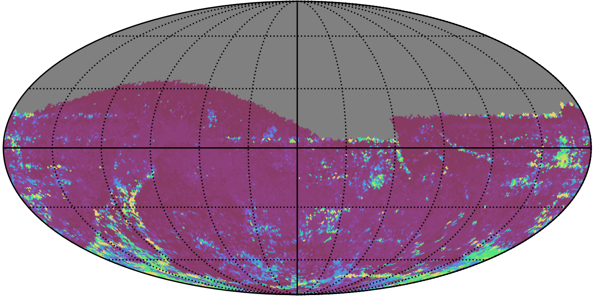
too_elab_heavy_r32_d2_griz_v3.4_10yrs All sky z band: 75th Percentile Intranight Timespan
