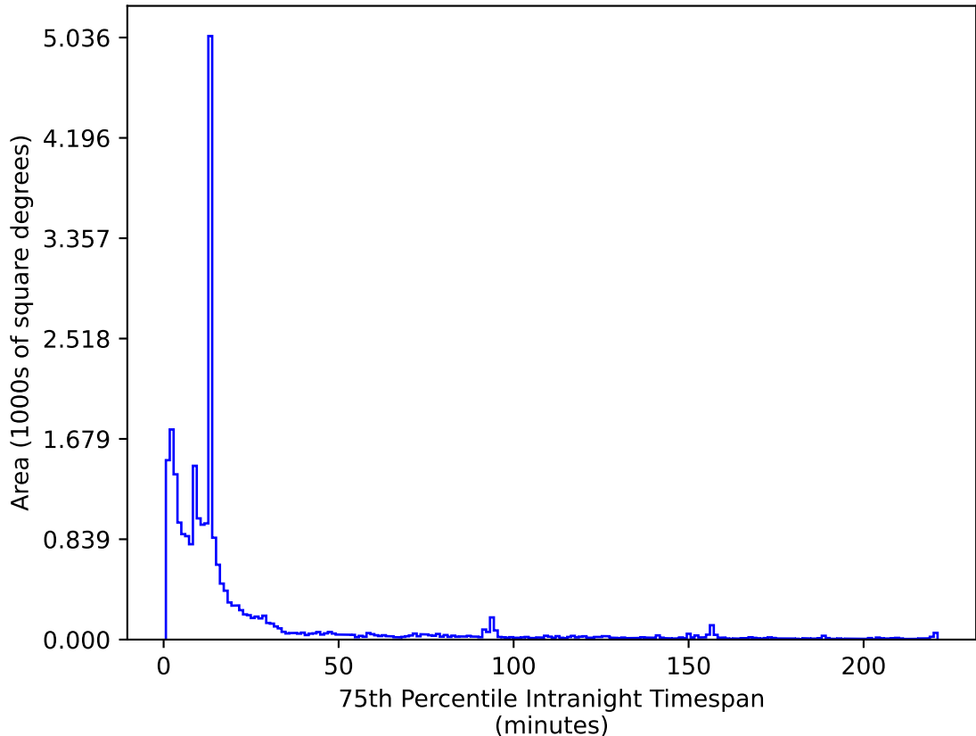
too_elab_heavy_r32_d2_griz_v3.4_10yrs All sky z band: 75th Percentile Intranight Timespan
