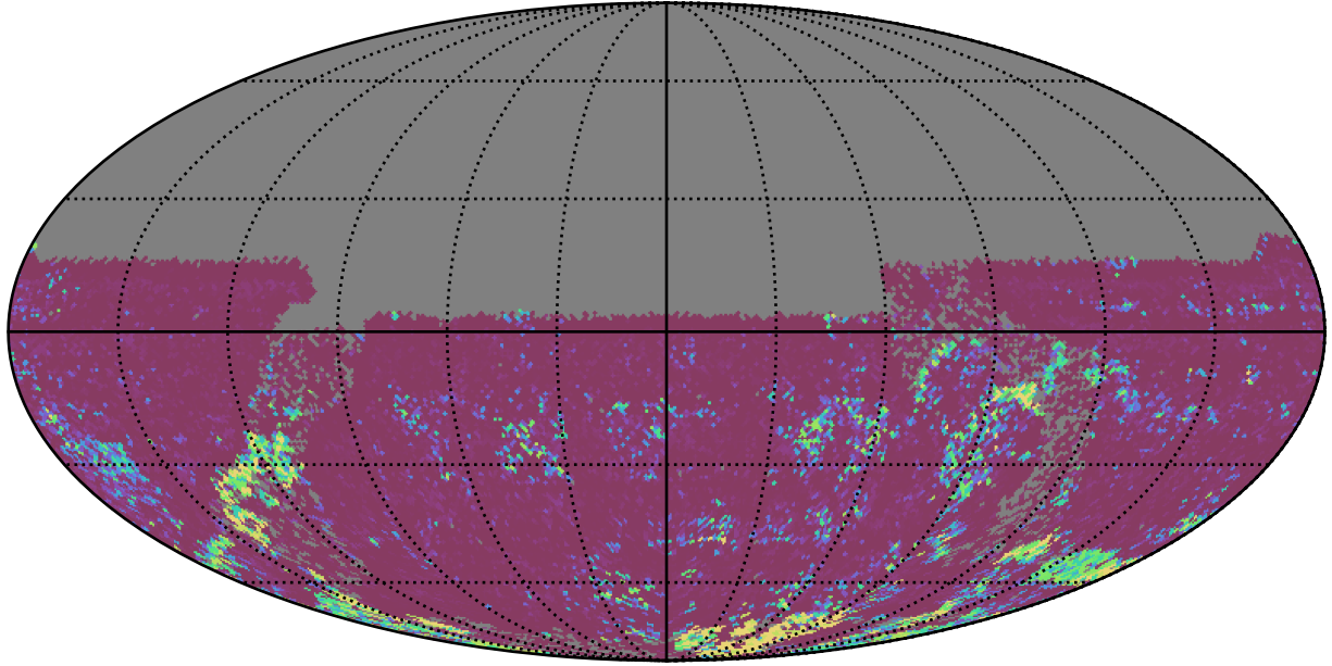
too_elab_heavy_r32_d2_griz_v3.4_10yrs All sky u band: 75th Percentile Intranight Timespan
